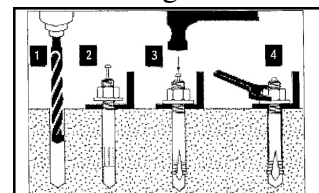
Anchor Bolt Diagram
